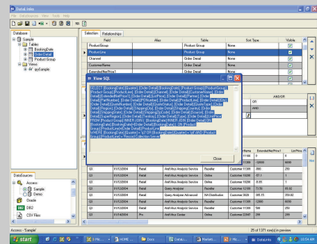
DataLinks™ Pro SQL Writer.
